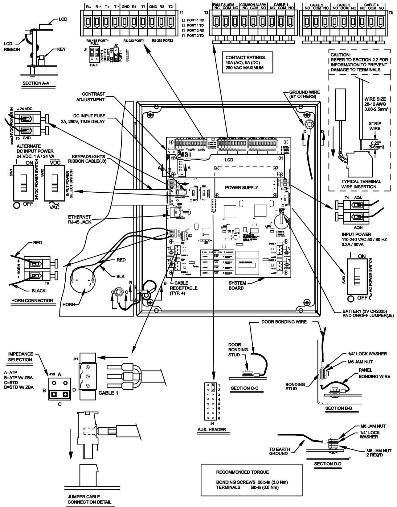
Figure 2-3 Wiring Diagram for PAL-AT Model AT30K
